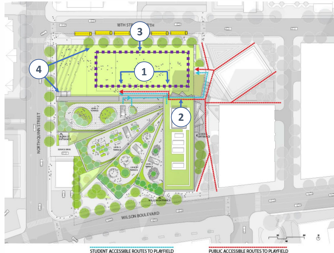
Field Elevation at 175' – Student and Public Accessible Routes
