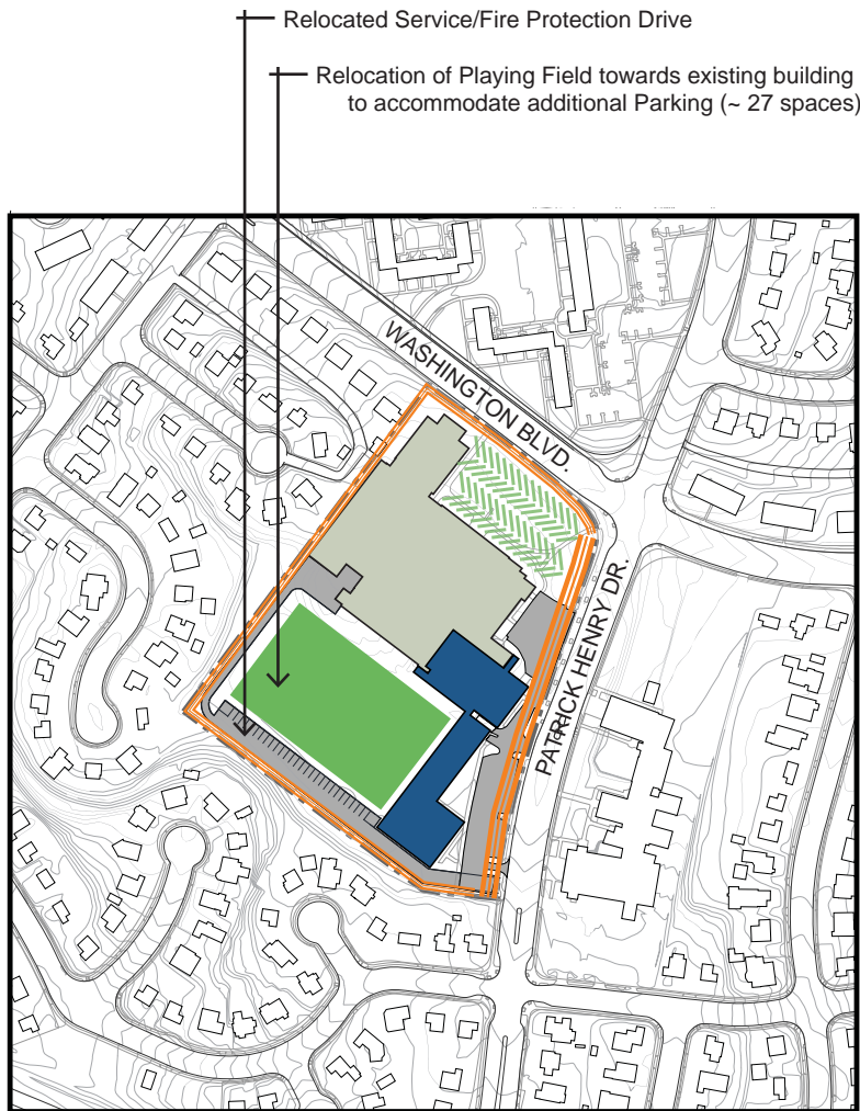
Zoning and Site Constraints Plan
