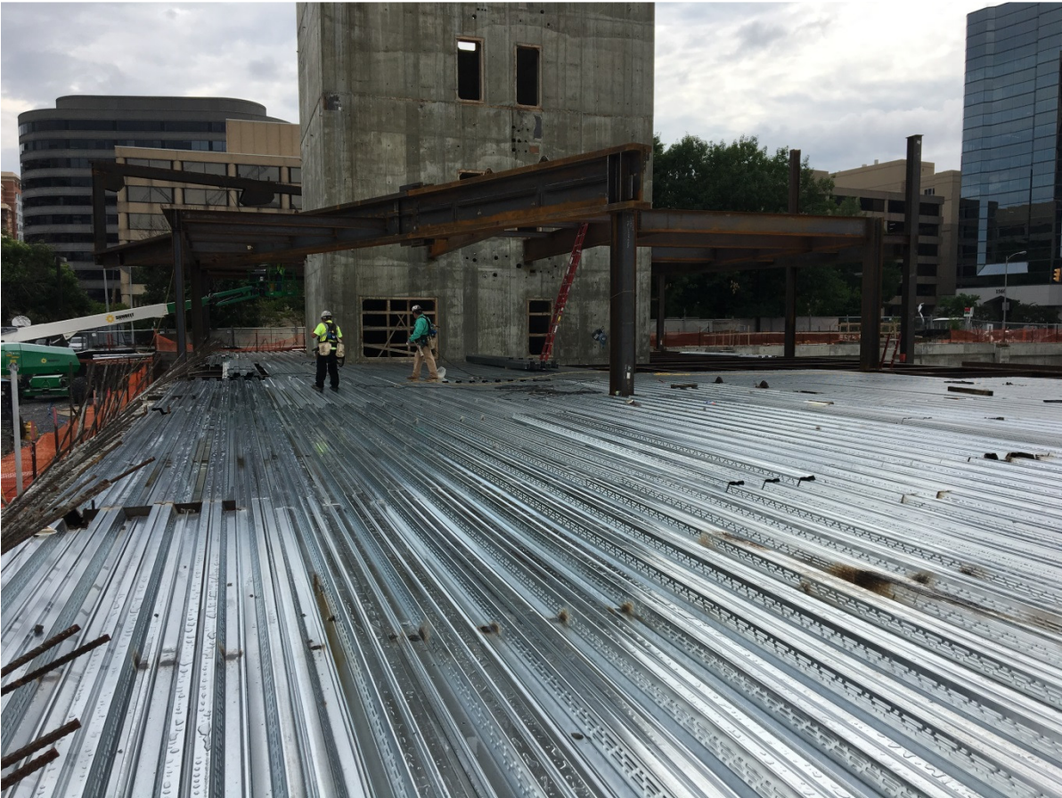
Metal decking @ Level 1
